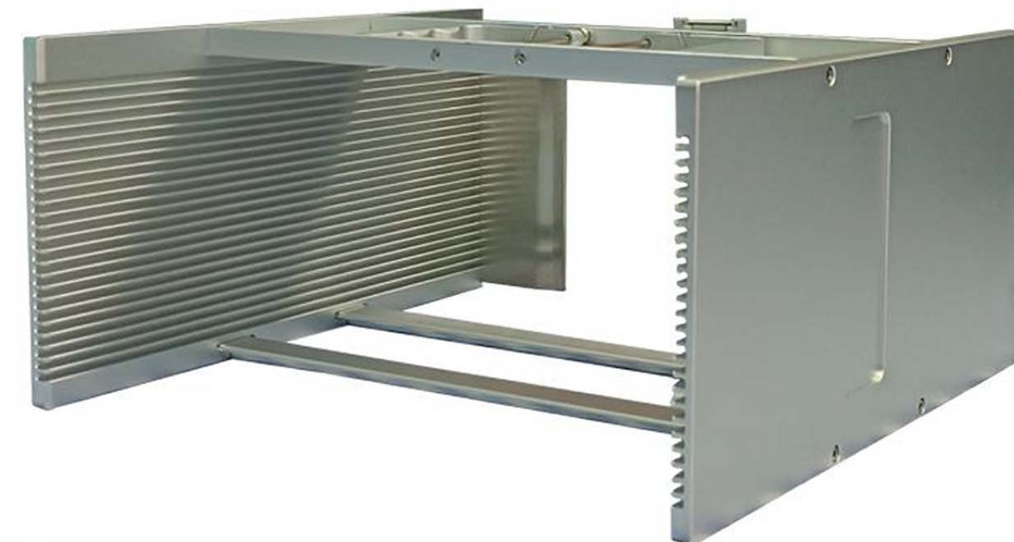
6" 25 slots of square iron ring cassette, F06 type Art. No: DSF24F06 Size : 207x215x144 mm
