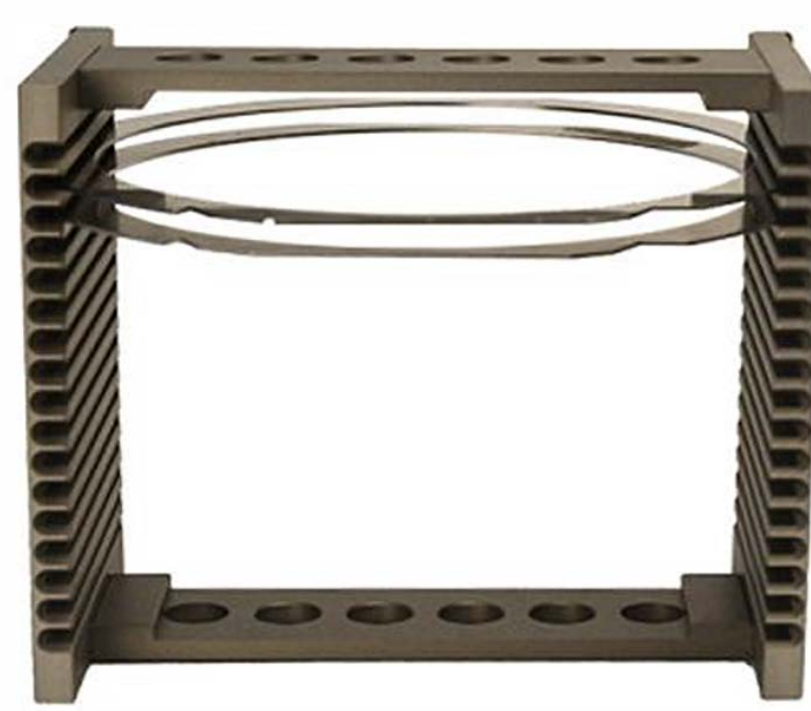
6" non-standard cassette,A26 type Art. No.: DSF20A26-000-R0 Size: 222×120×180 mm
