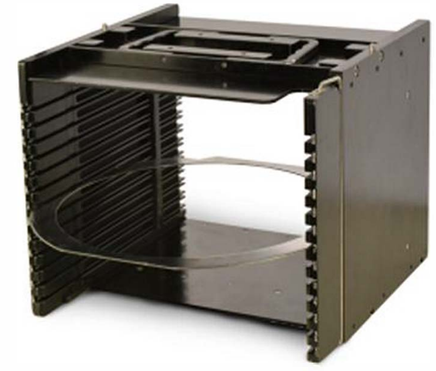
8" 13 slots of cassette, I08 type Art. No: DSF20I08 Size: 276x288x205 mm
