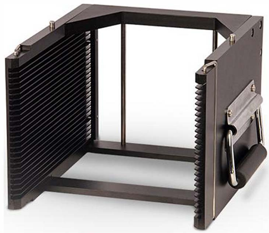
5" 25 slots of cassette,E05 type Art. No.: DSF20E05 Size: 177.8×205×142.8 mm
