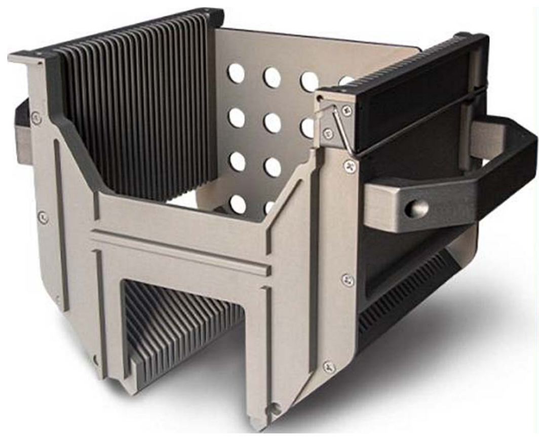
8" 25 slots of wafer cassette,A58 type Art. No.: DSF21A58 Size: 223×203.3×215.05 mm Material: AL 7075 DIST: 4.76mm Wide: 3.5mm Depth: 13.5mm
