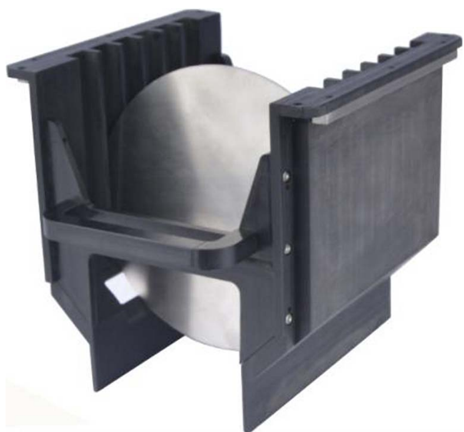
6" 6 slots of wafer cassette,I06 type Art. No.: DSF20J06 Size: 179x171x167.7 mm (Material): Black ESD POM (Slot distance): 19mm (Slot width): 15mm (Slot depth): 9.5mm
